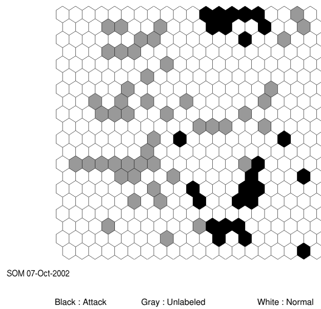
Figure 5.12: Neuron Labels of the neuron 4 third level map
