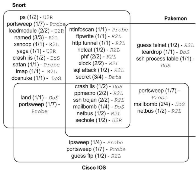
Figure 2.4: Analysis of detected attacks
