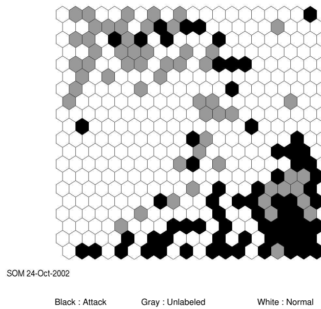
Figure 5.21: Neuron Labels of the neuron 23 third level map
