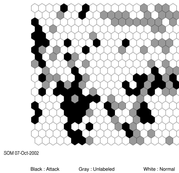
Figure 5.15: Neuron Labels of the neuron 17 third level map
